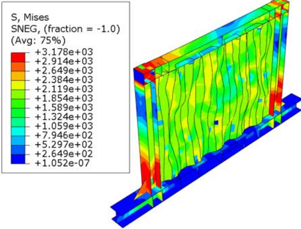
Fig. 6 Comparison of the failure mode of the test, and Von Mises stress of the FE modeling.
