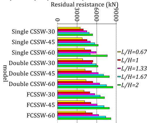
Fig. 16 Comparative analysis of the residual resistance exhibited by the numerical models.
