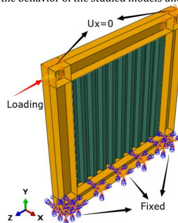
Fig. 4 Numerical model boundary constraints and lateral load arrangement
