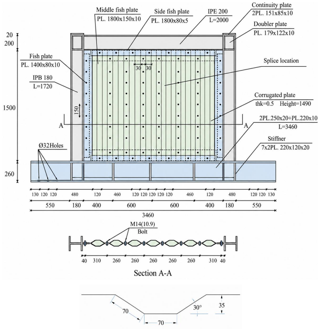
Fig. 7 The geometric features of the vertical DCSSWs test.
