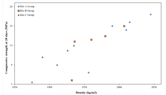
Fig. 9 Relationships between density and compressive strength in pervious concrete
