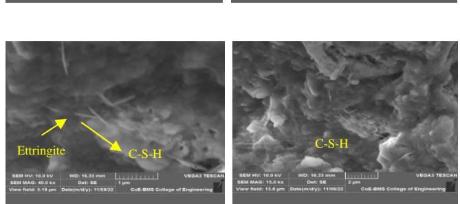
Fig. 3 SEM images of Graphene oxide concrete at 28 days
