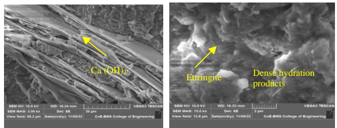
Fig. 2 SEM images of conventional concrete at 28 days
