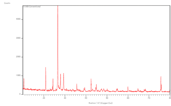
Fig. 4 XRD for conventional concrete specimen
