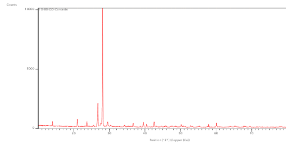
Fig. 5 XRD for Graphene oxide concrete specimen
